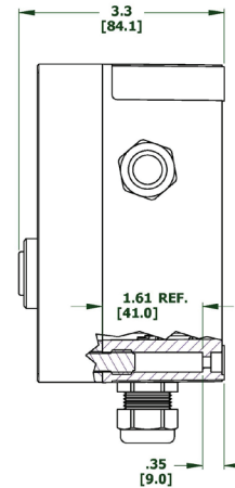
CP-10 Controller
